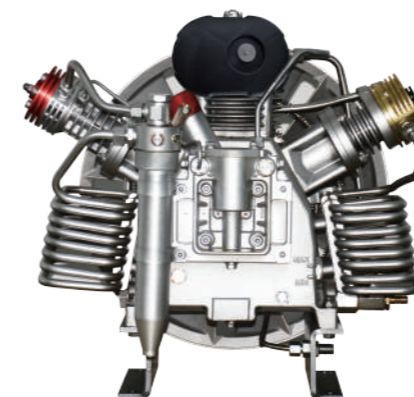
Compressor block
